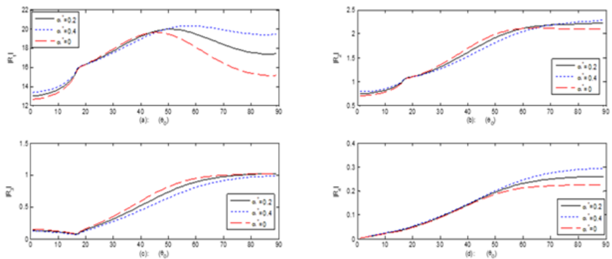
Figure 8. (a, b, c, d): TDP effects on amplitude ratios for an incident T -wave.
