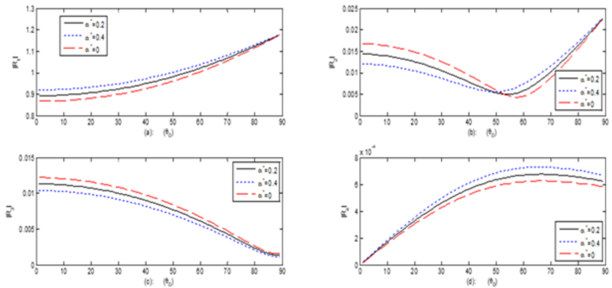
Figure 7. (a, b, c, d): TDP effects on amplitude ratios for an incident P -wave.
