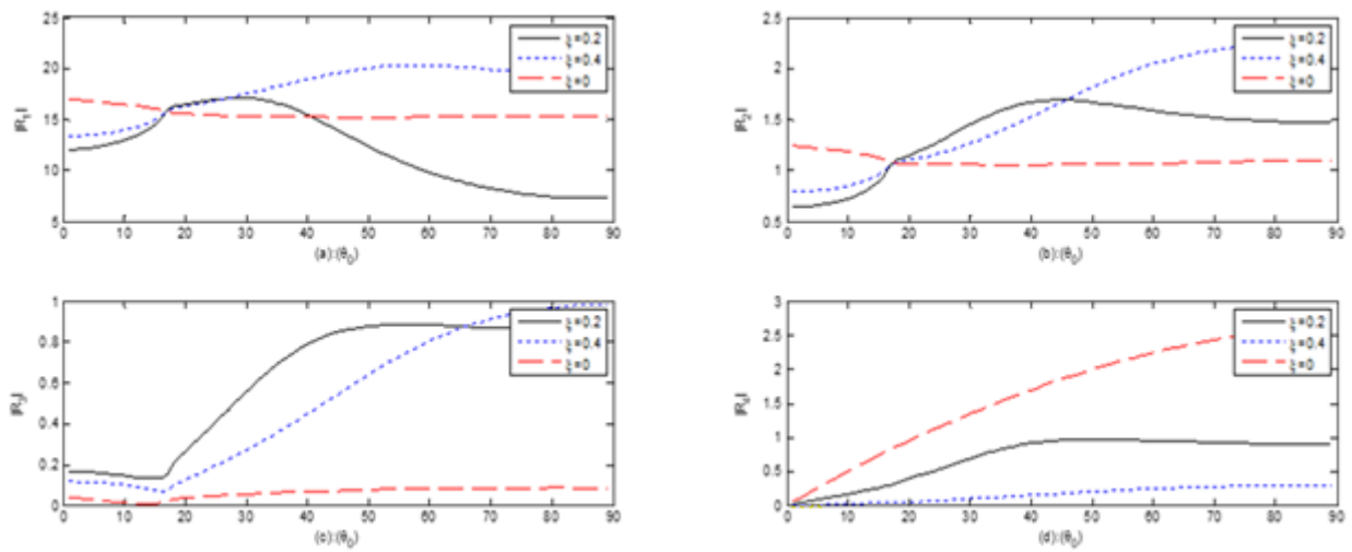
Figure 11. (a, b, c, d): Nonlocal influence on amplitude ratios for an incident T -wave.
