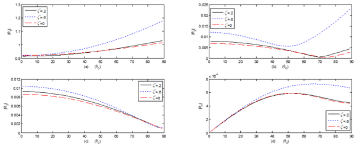
Figure 1. (a, b, c, d): HTT effects on amplitude ratios for an incident P -wave
