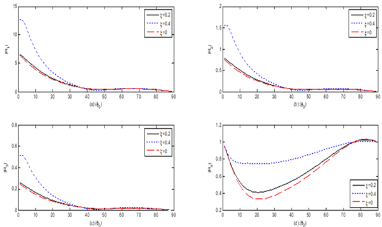
Figure 12. (a, b, c, d): Nonlocal influence on amplitude ratios for an incident SV -wave.
