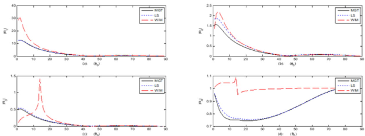
Figure 6. (a, b, c, d): Impedance and thermoelastic-model effects on amplitude ratios for an incident SV -wave.
