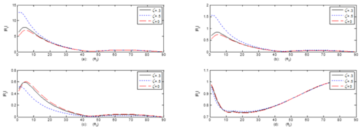
Figure 3. (a, b, c, d): HTT effects on amplitude ratios for an incident SV -wave
