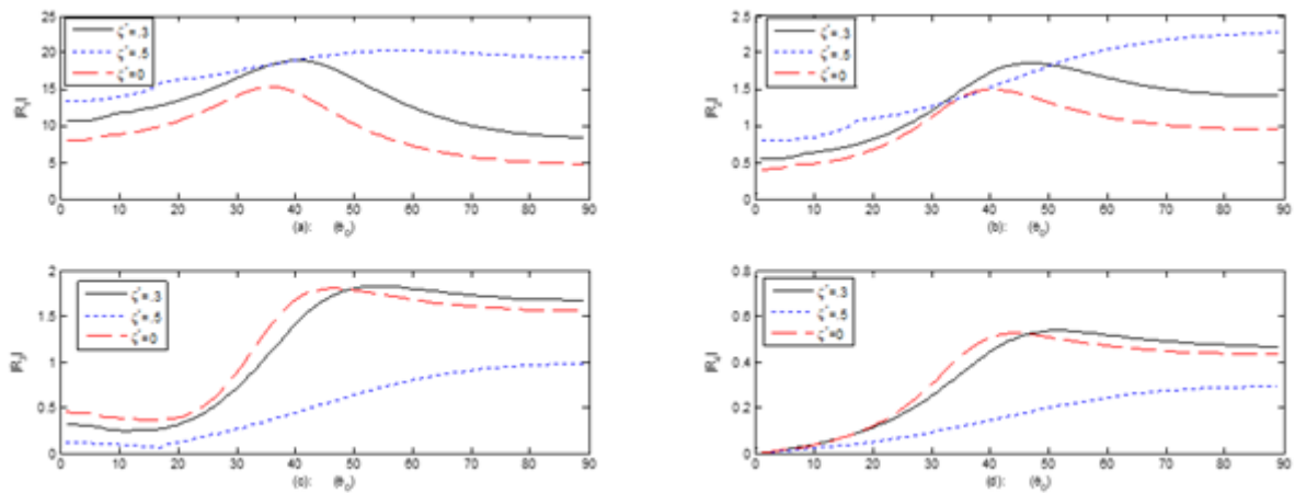
Figure 2. (a, b, c, d): HTT effects on amplitude ratios for an incident T -wave
