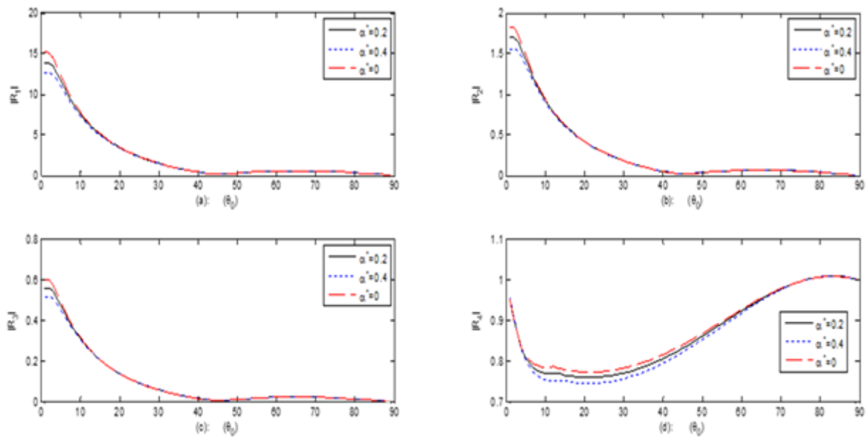
Figure 9. (a, b, c, d): TDP effects on amplitude ratios for an incident S V-wave.
