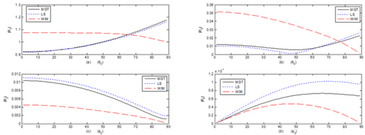
Figure 4. (a, b, c, d): Impedance and thermoelastic-model effects on amplitude ratios for an incident P -wave
