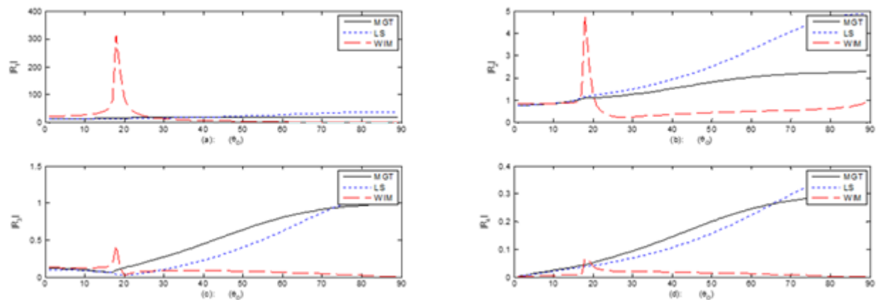
Figure 5. (a, b, c, d): Impedance and thermoelastic-model effects on amplitude ratios for an incident T -wave.
