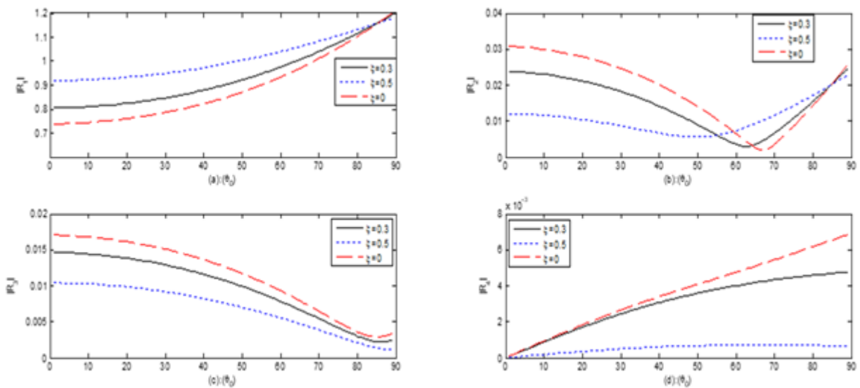
Figure 10. (a, b, c, d): Nonlocal influence on amplitude ratios for an incident P -wave.
