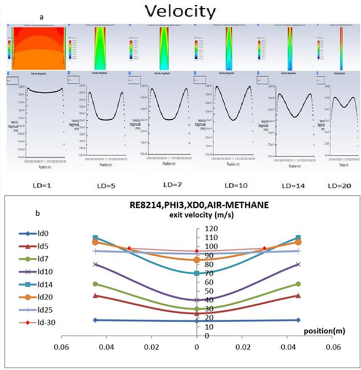
Figure 6. Exit velocity distribution profiles of the burner at varying mixing lengths (LD).(a).CFD model flow field ,(b) quantitative analysis for mixing field
