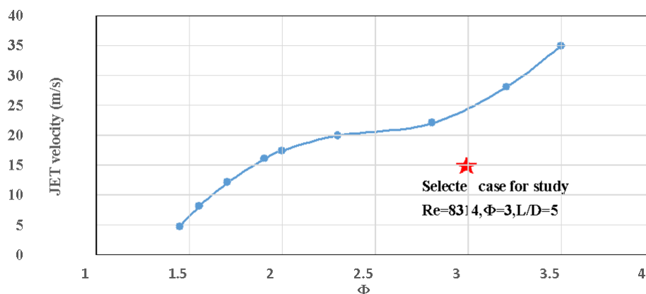
Figure 4. Represent the stability curve of CFCB at LD = 5, the red circle represent selected case study
