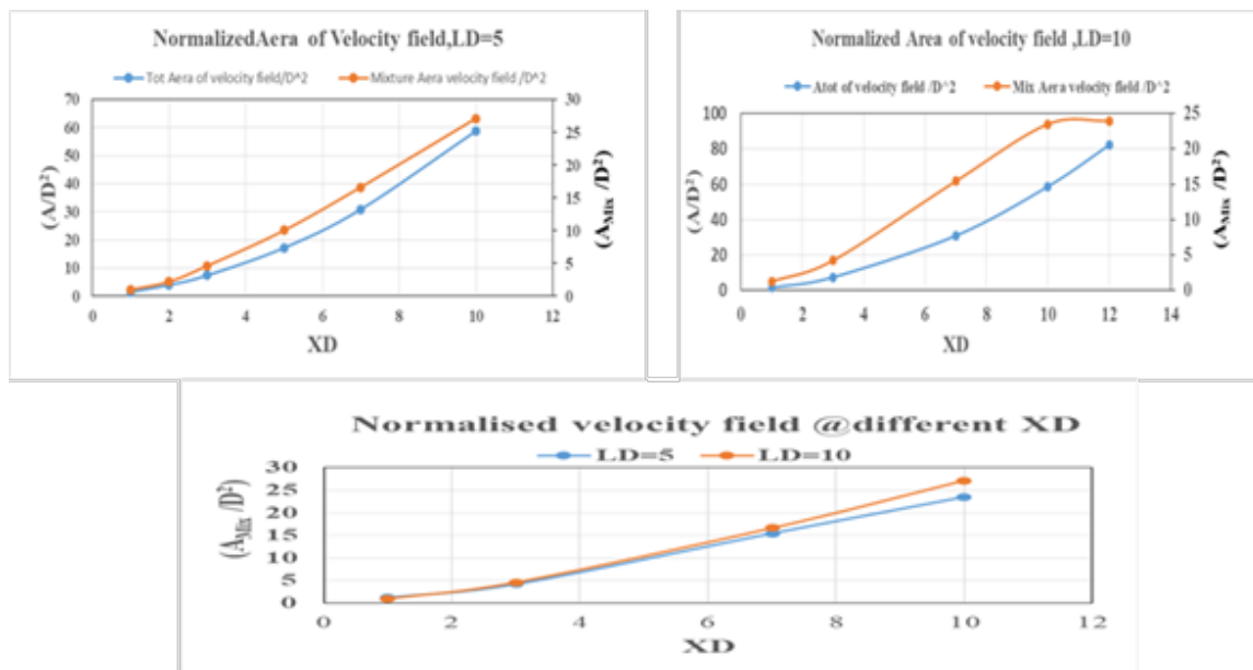
Figure 9. represent mixture area percent according total mixing field for different LD =5,LD=10
