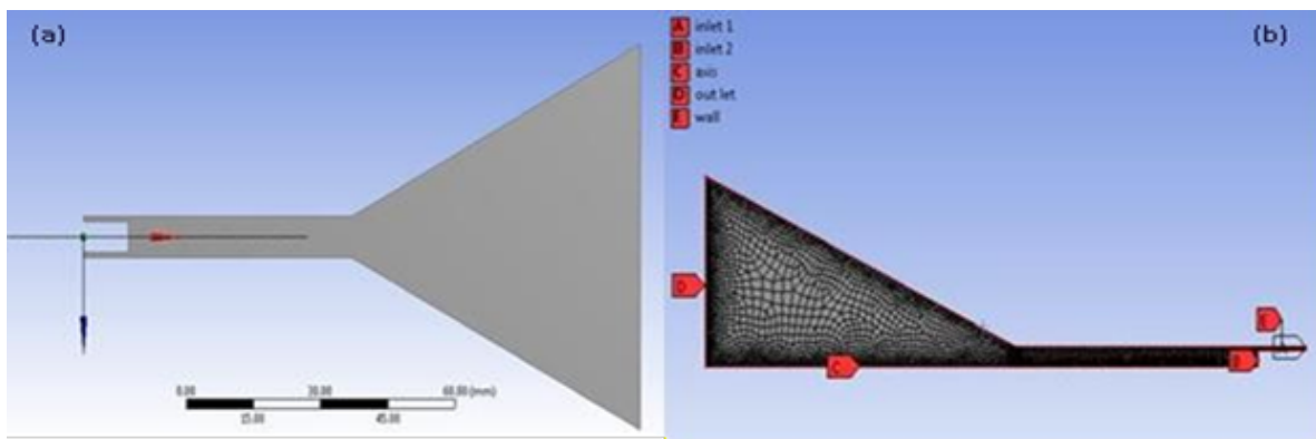
Figure 2. (a) geometry of burner with conical section, (b) mesh and inputs of study
