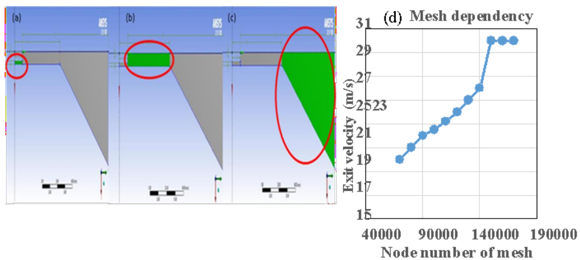
Figure 3. (a)-represent the inlet of fuel (b) represent the inlet of air and mixing length LD (c) represent the conical section with certain XD, (d) mesh sensitivity
