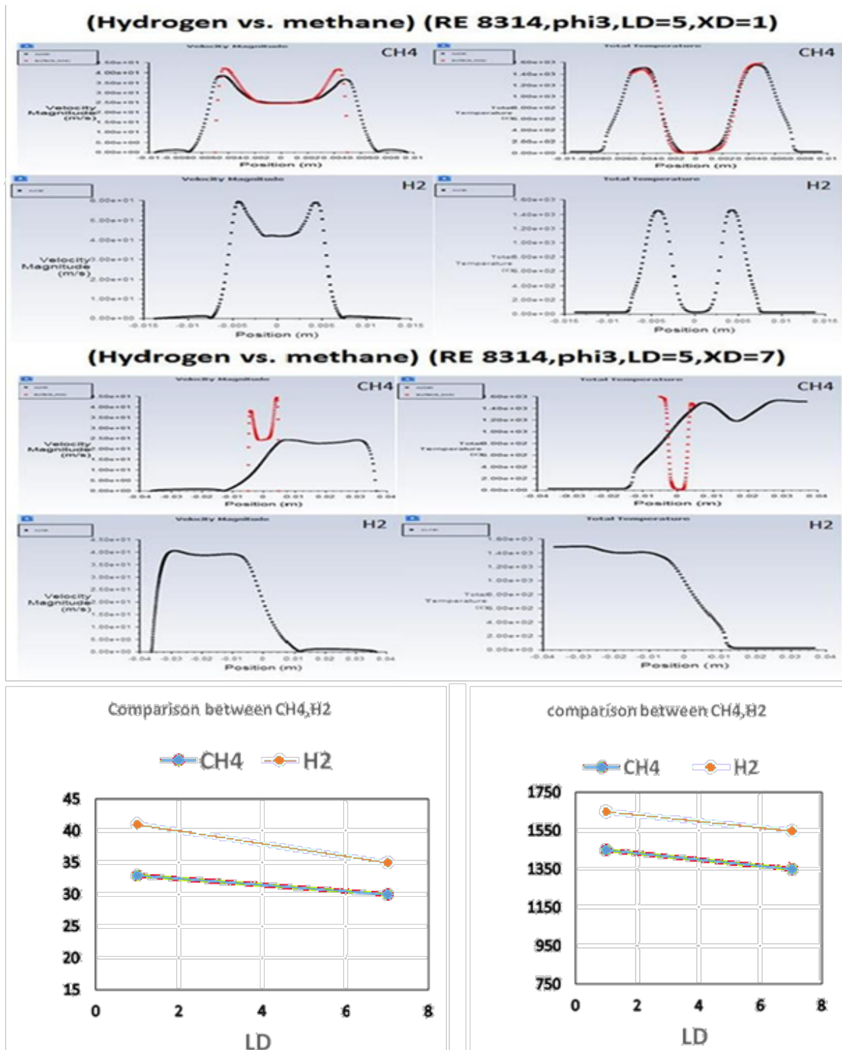
Figure 12. fuel type effect, comparison between velocity and temperature for hydrogen and methane
