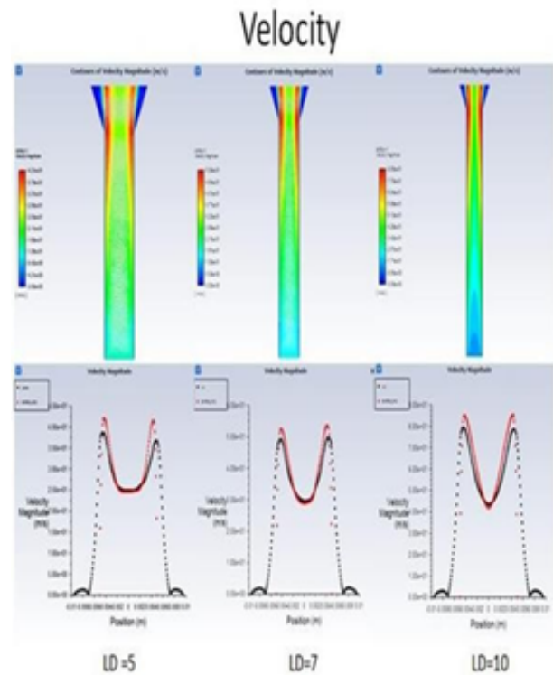
Figure 8. comparison between different LD at XD=1
