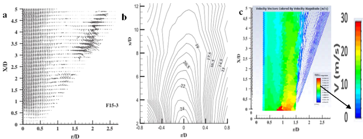
Figure 5. (a) illustrate experimental PIV recirculation eddies that make stabilization mechanism in burner, (b) represent stream lines contours for same region (c): represent the shape of same region extracted from CFD results
