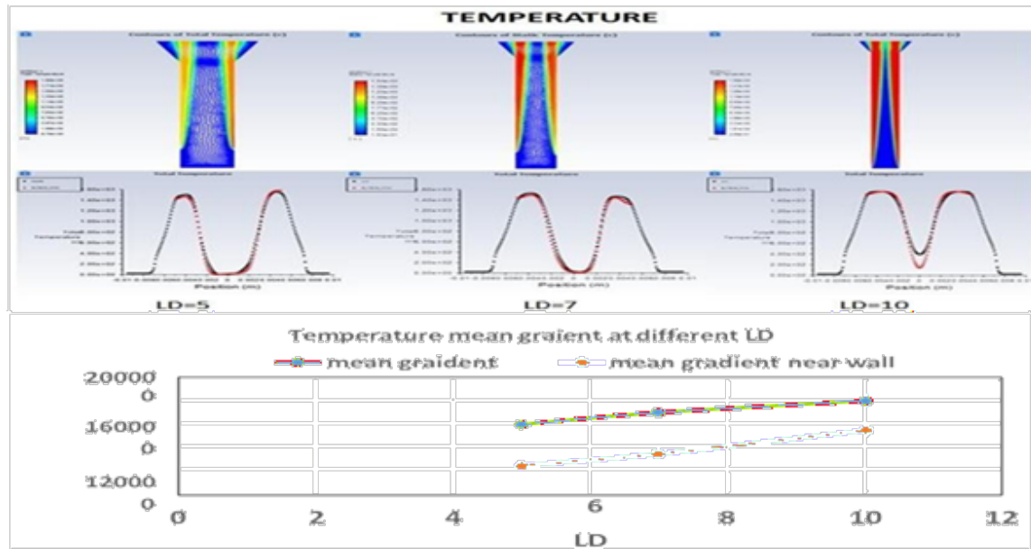
Figure 11. Illustrate temperature profiles distribution for XD=1 & different LD
