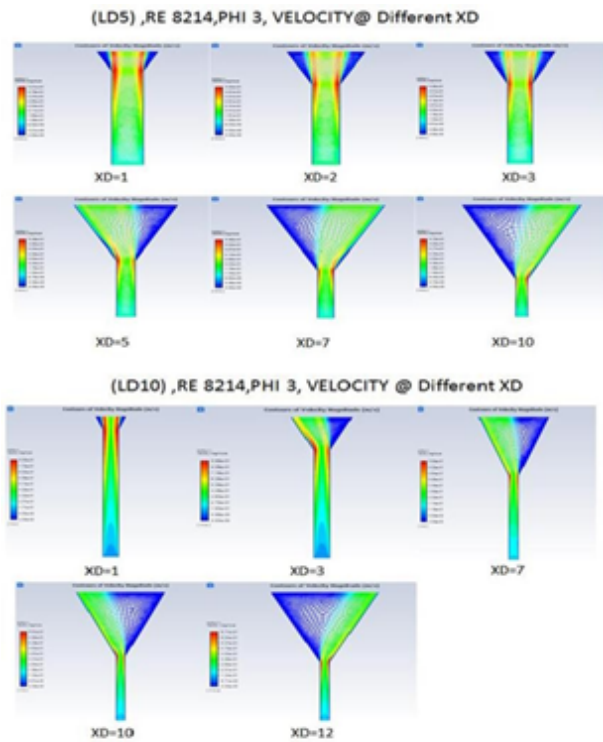
Figure 7. comparison between different LD = 5 & 10 for different XD
