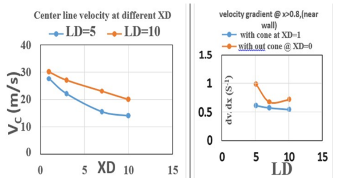
Figure 10. (a) center velocity for different XD, (b) gradient of velocity near wall for different LD with and without cone
