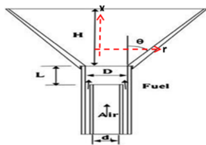
(a) Dimensions of burner
