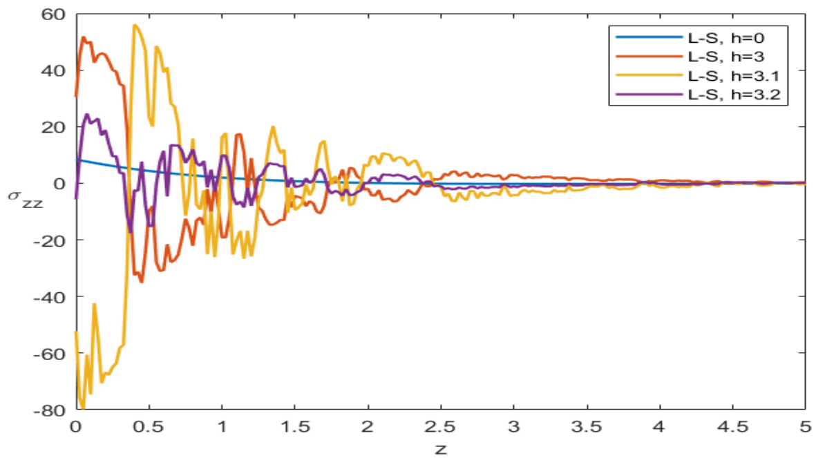
Figure 20. The stress tensor ( \sigma_{zz} ) distributions for the L-S theory
