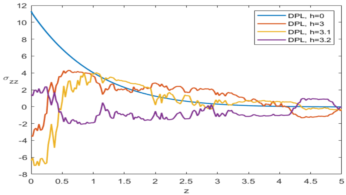
Figure 13. The stress tensor ( \sigma_{zz} ) distributions for the DPL model
