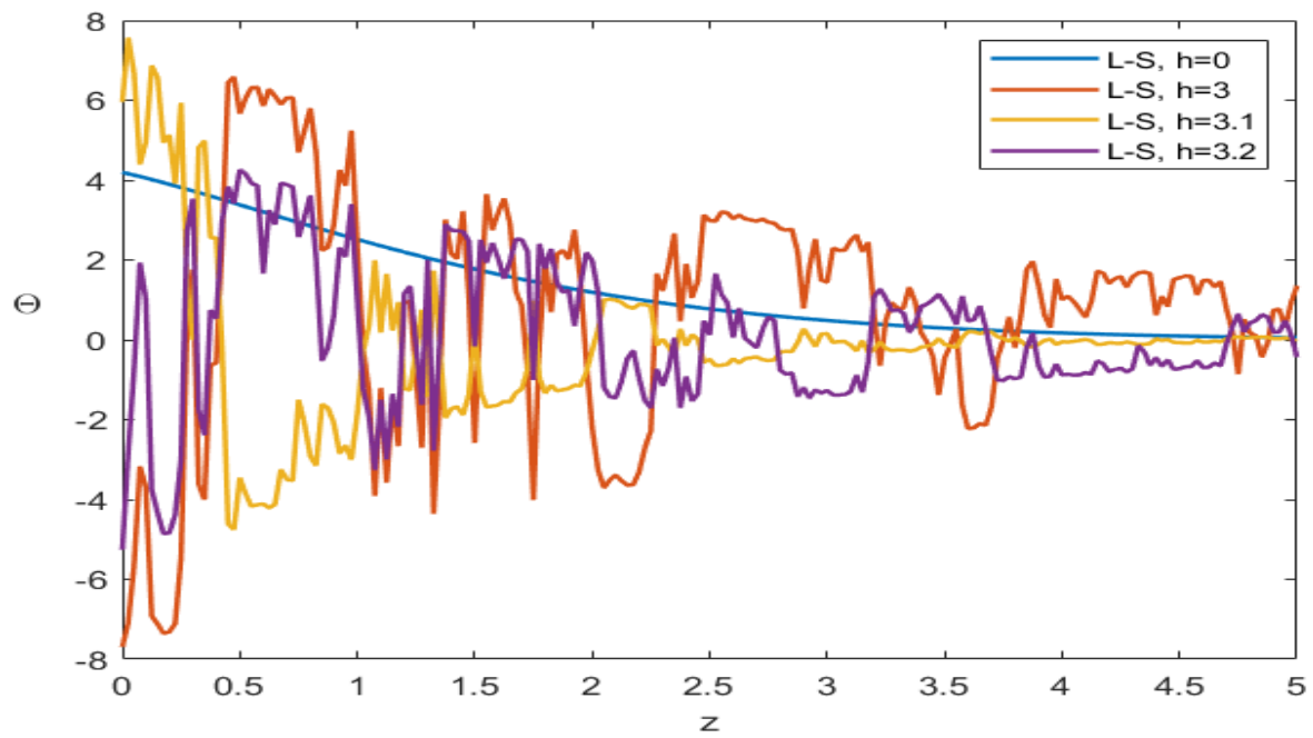
Figure 17. The temperature distributions for the L-S theory
