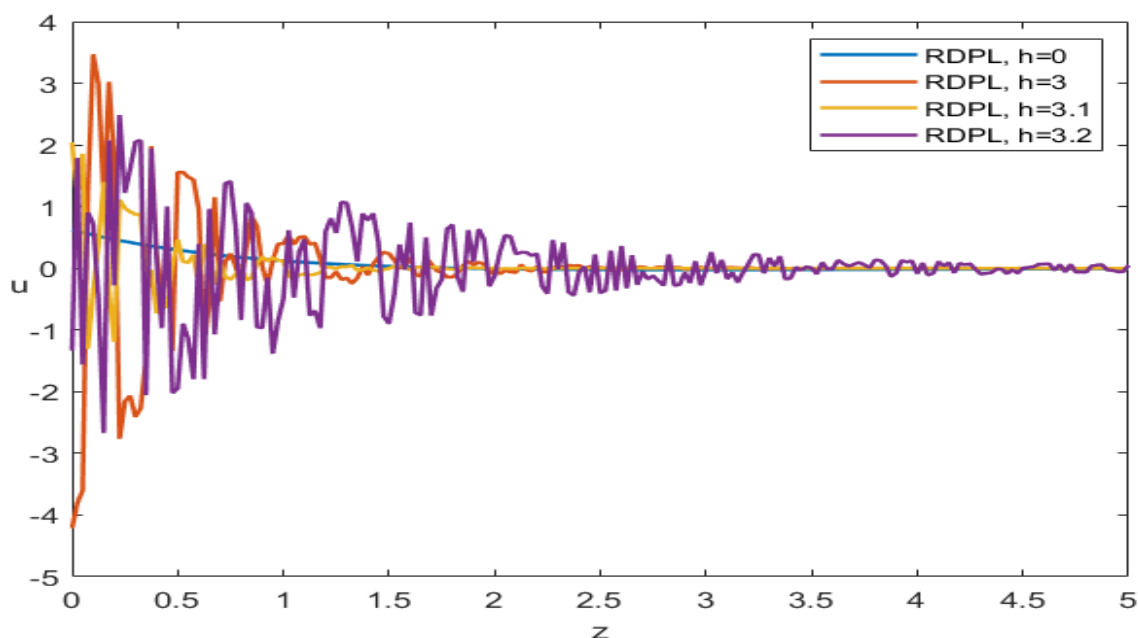
Figure 1. The horizontal displacement distributions for the RDPL model
