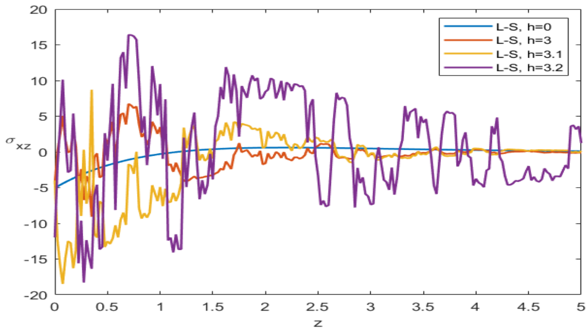
Figure 21. The stress tensor ( \sigma_{xz} ) distributions for the L-S theory
