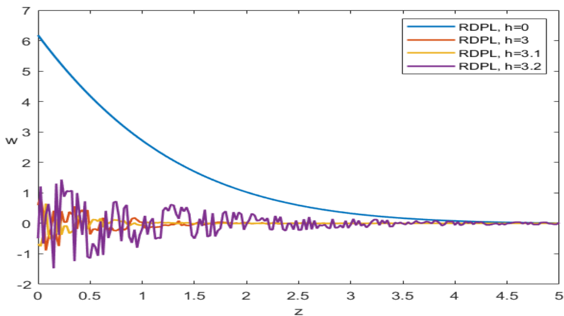
Figure 2. The vertical displacement distributions for the RDPL model
